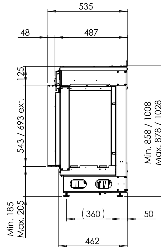
Dimensional Drawing e-MatriX Mood 800/500 I + e-MatriX Mood 800/650 I
